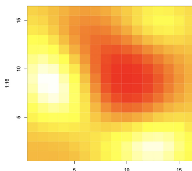
Composite basis functions (Araki et al. 2019): Basis functions with sparse singular value decomposition
